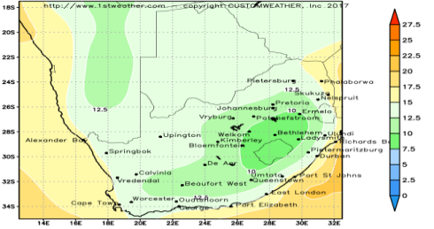
GFS 50KM MAXIMUM TEMPERATURE (C) INIT: 12UTC 02JUN19 VALID: MON 03 JUN 2019
