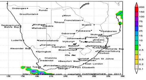
GFS 50KM POSSIBLE 24-HOUR RAINFALL (mm) INIT: 12UTC 02JUN19 VALID: 02H00 MON 03 JUN - 02H00 TUE 04 JUN
