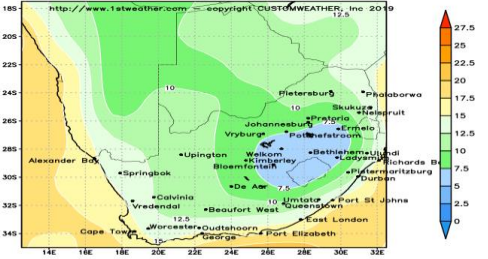
GFS 50KM MAXIMUM TEMPERATURE (C) INIT: 18UTC 18JUN19 VALID: WED 19 JUN 2019
