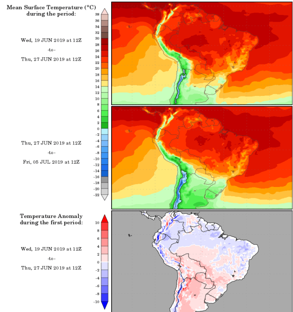
Temperature forecasts from the National Centers for Environmental Prediction. Normal Temperature derived from CRU monthly climatology for 1901-2000. Forecast Initialization Time: 12Z18JUN2019
