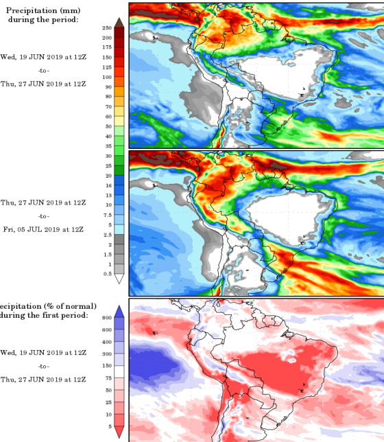
Precipitation forecasts from the National Centers for Environmental Prediction. Normal rainfall derived from Xie-Arkin (CMAP) Monthly Climatology for 1979-2003. Forecast Initialization Time: 12Z18JUN2019
