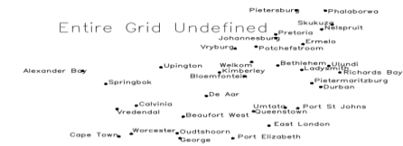
GFS 50KM MAXIMUM TEMPERATURE (C) INIT: 18UTC 06JUN19 VALID: FRI 07 JUN 2019 http://www.1stweather.com - copyright CUSTOMWEATHER, Inc 2017
