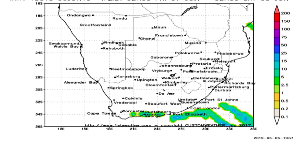
GFS 50KM POSSIBLE 24-HOUR RAINFALL (mm) INIT: 18UTC 06JUN19 VALID: 02H00 FRI 07 JUN - 02H00 SAT 08 JUN
