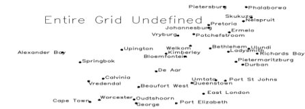
GFS 50KM POSSIBLE 24-HOUR RAINFALL (mm) INIT: 18UTC 06JUN19 VALID: 02H00 FRI 07 JUN - 02H00 SAT 08 JUN
