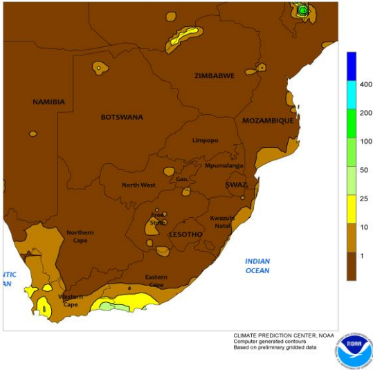
SOUTH AFRICA Total Precipitation (mm) July 14 - 20, 2019
