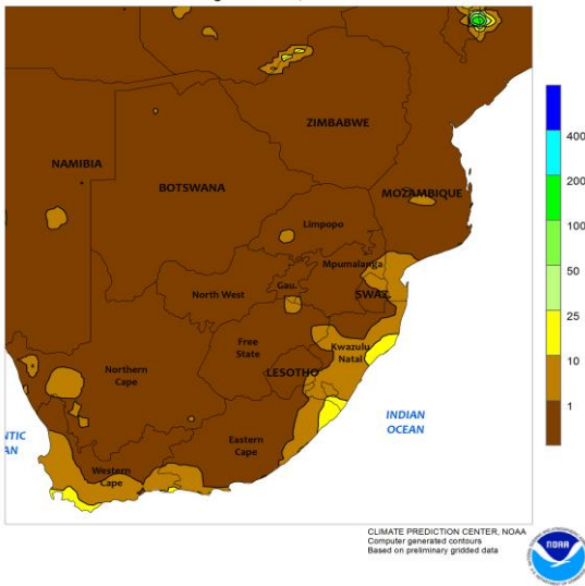
SOUTH AFRICA Total Precipitation (mm) August 25 - 31, 2019
