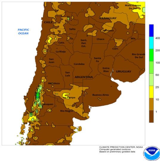
ARGENTINA Total Precipitation (mm) September 22 - 28, 2019
