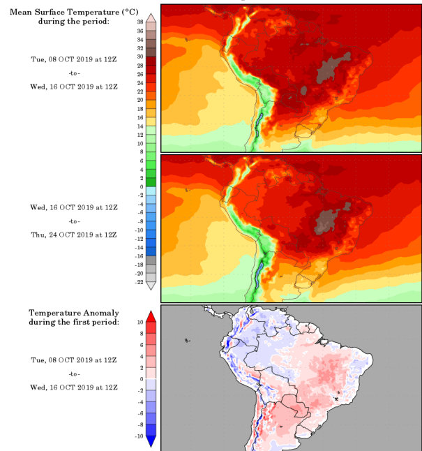
Temperature forecasts from the National Centers for Environmental Prediction. Normal Temperature derived from CRU monthly climatology for 1901-2000 Forecast Initialization Time: 12Z08OCT2019
