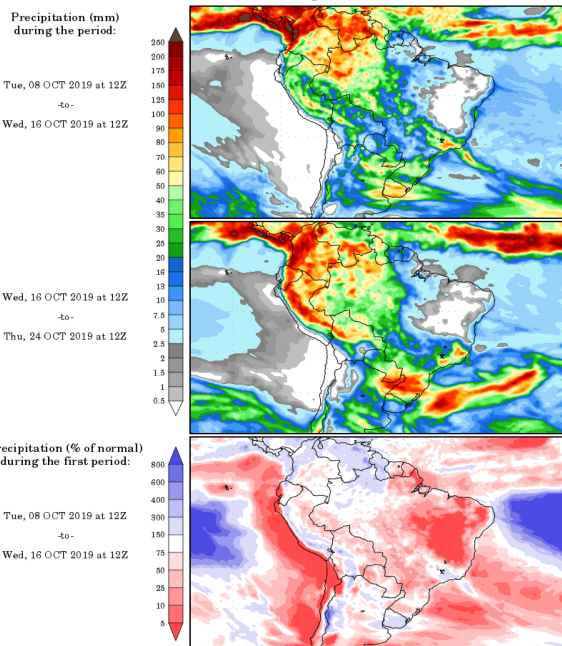
Precipitation forecasts from the National Centers for Environmental Prediction. Normal rainfall derived from Xie-Arkin (CMA) Monthly Climatology for 1978-2003. Forecast Initialization Time: 12Z08OCT2019
