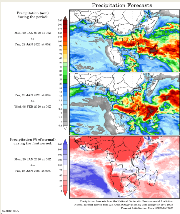
CLIMATE PREDICTION CENTER, NOAA Computer generated contours Based on preliminary gridded data
