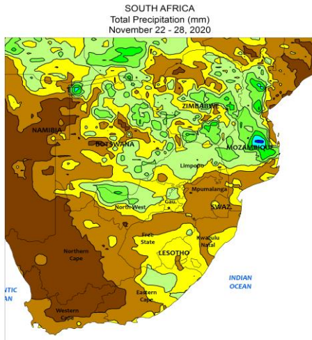
SOUTH AFRICA Total Precipitation (mm) November 22 - 28, 2020
