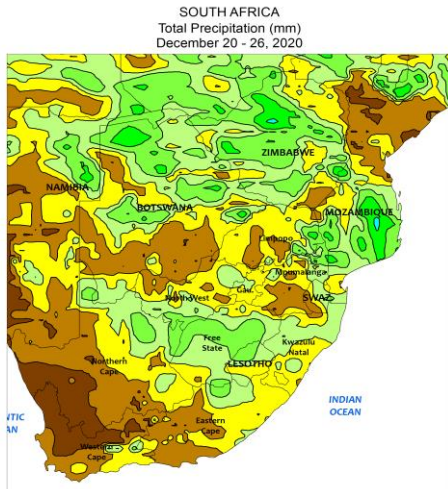
SOUTH AFRICA Total Precipitation (mm) December 20 - 26, 2020 CLIMATE PREDICTION CENTER, NOAA Computer generated contour Based on preliminary gridded data
