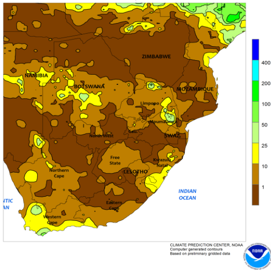
SOUTH AFRICA Total Precipitation (mm) March 7 - 13, 2021
