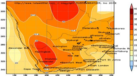
GFS 50KM MAXIMUM TEMPERATURE (C) INIT: 18UTC 22MAR21 VALID: TUE 23 MAR 2021
