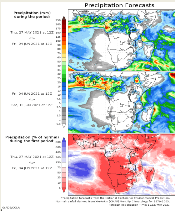
CLIMATE PREDICTION CENTER, NOAA Computer generated contour. NOAA Based on preliminary gridded data
