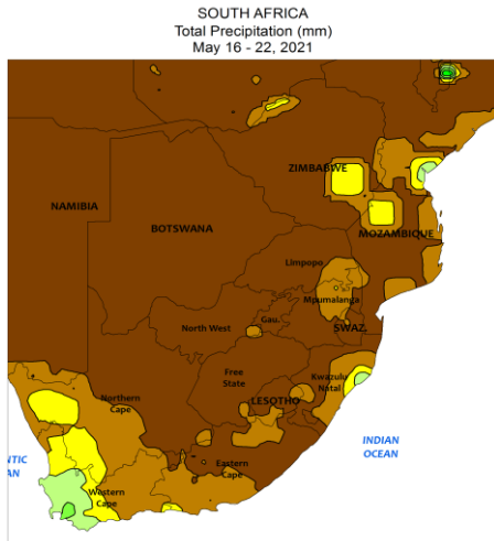
CLIMATE PREDICTION CENTER, NOAA Computer generated contour. NOAA Based on preliminary gridded data
