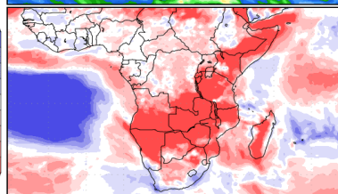
Precipitation forecasts from the National Centers for Environmental Prediction. Normal rainfall derived from Xie-Arkin (CMAP) Monthly Climatology for 1979-2003. Forecast Initialization Time: 12Z24AUG2021
