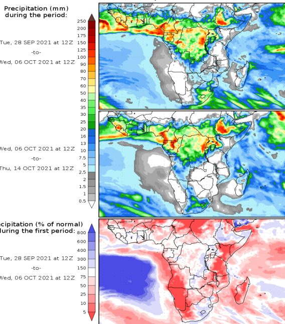
Precipitation forecasts from the National Centers for Environmental Prediction. Normal rainfall derived from Xie-Arkin (CMAP) Monthly Climatology for 1979-2003. Forecast Initialization Time: 12Z28SEP2021
