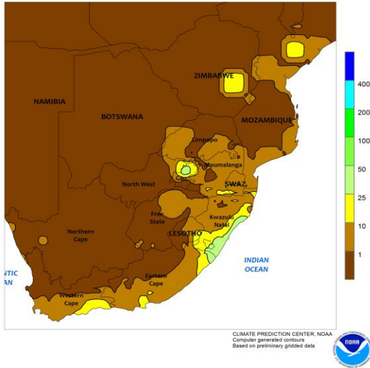
SOUTH AFRICA Total Precipitation (mm) September 12 - 18, 2021
