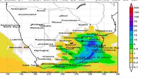
GFS 50KM POSSIBLE 24-HOUR RAINFALL (mm) INIT: 18UTC 28SEP21 VALID: 20H00 TUE 28 SEP - 20H00 WED 29 SEP
