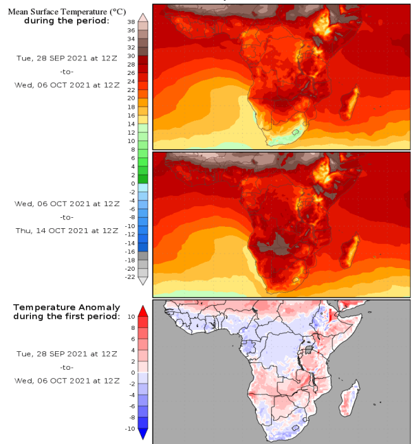
Temperature forecasts from the National Centers for Environmental Prediction. Normal Temperature derived from CRU monthly climatology for 1901-2000 Forecast Initialization Time: 12Z28SEP2021
