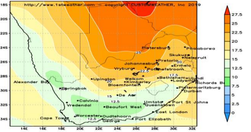
GFS 50KM MAXIMUM TEMPERATURE (C) INIT: 18UTC 28SEP21 VALID: WED 29 SEP 2021
