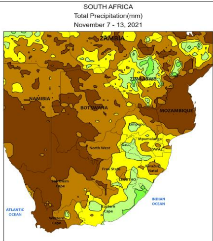
SOUTH AFRICA Total Precipitation (mm) November 7 - 13, 2021 CLIMATE PREDICTION CENTER, NOAA Computer generated contours Based on preliminary data
