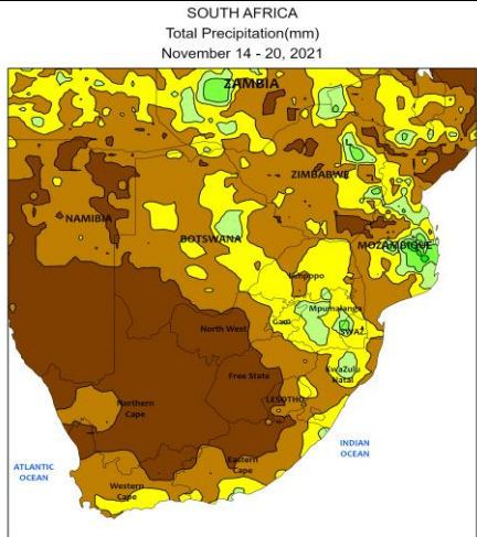
SOUTH AFRICA Total Precipitation(mm) November 14 - 20, 2021 CLIMATE PREDICTION CENTER, NOAA Computer generated contours Based on preliminary data
