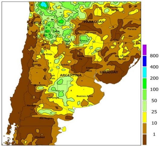
ARGENTINA Total Precipitation(mm) December 19 - 25, 2021
