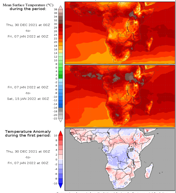
Temperature forecasts from the National Centers for Environmental Prediction. Normal Temperature derived from CRU monthly climatology for 1901-2000 Forecast Initialization Time: 00Z30DEC2021
