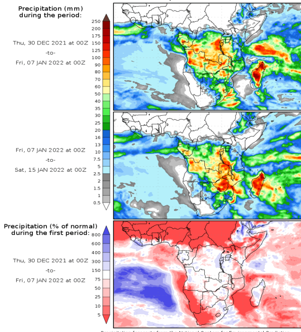
Precipitation forecasts from the National Centers for Environmental Prediction. Normal rainfall derived from Xie-Arkin (CMAP) Monthly Climatology for 1979-2003. Forecast Initialization Time: 00Z30DEC2021
