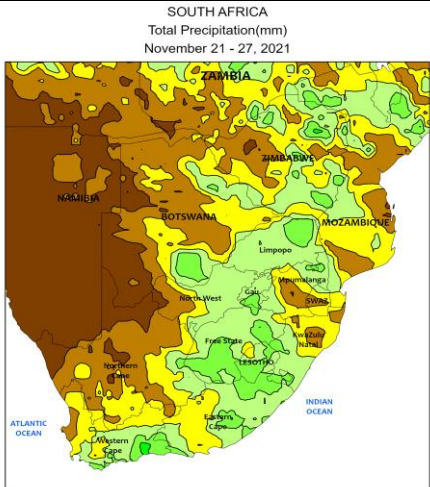
SOUTH AFRICA Total Precipitation (mm) November 21 - 27, 2021 CLIMATE PREDICTION CENTER, NOAA Computer generated contours Based on preliminary data
