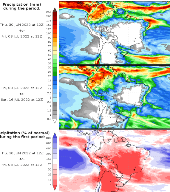
Precipitation forecasts from the National Centers for Environmental Prediction. Normal rainfall derived from Xie-Arkin (CMAP) Monthly Climatology for 1979-2003. Forecast Initialization Time: 12Z30JUN2022
