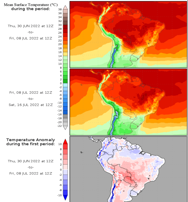
Temperature forecasts from the National Centers for Environmental Prediction. Normal Temperature derived from CRU monthly climatology for 1901-2000 Forecast Initialization Time: 12Z30JUN2022
