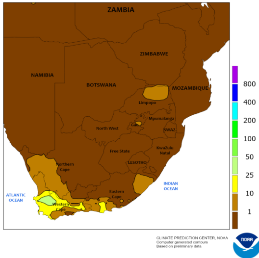
SOUTH AFRICA Total Precipitation(mm) September 4 - 10, 2022
