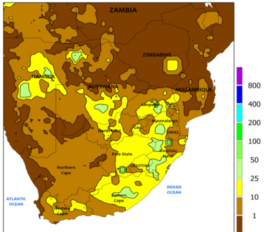
SOUTH AFRICA Total Precipitation(mm) October 16 - 22, 2022
