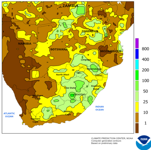
SOUTH AFRICA Total Precipitation(mm) October 30 - November 5, 2022
