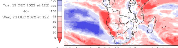
Precipitation forecasts from the National Centers for Environmental Prediction. Normal rainfall derived from Xie-Arkin (CMAP) Monthly Climatology for 1979-2003. Forecast Initialization Time: 12Z13DEC2022
