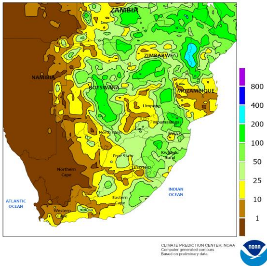
SOUTH AFRICA Total Precipitation(mm) February 12 - 18, 2023
