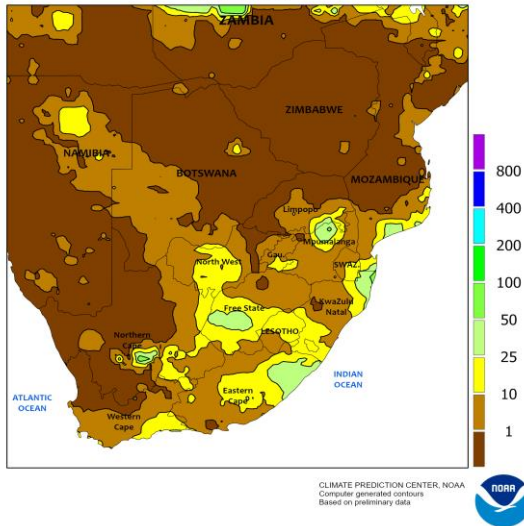
SOUTH AFRICA Total Precipitation(mm) April 2 - 8, 2023
