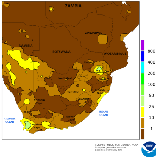
SOUTH AFRICA Total Precipitation(mm) April 23 - 29, 2023
