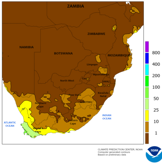
SOUTH AFRICA Total Precipitation(mm) May 21 - 27, 2023
