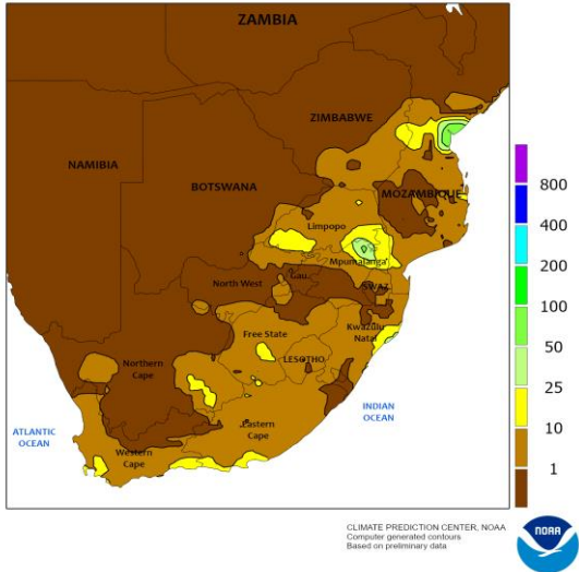
SOUTH AFRICA Total Precipitation(mm) July 16 - 22, 2023
