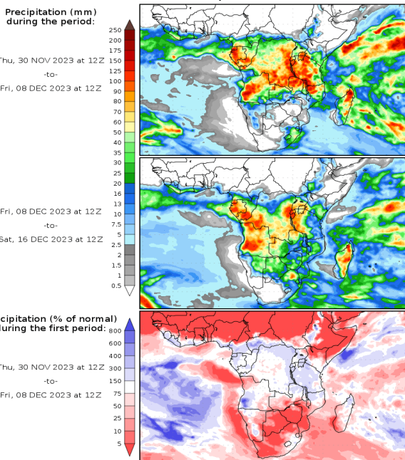
Precipitation forecasts from the National Centers for Environmental Prediction. Normal rainfall derived from Xie-Arkin (CMAP) Monthly Climatology for 1979-2003. Forecast Initialization Time: 12Z30NOV2023
