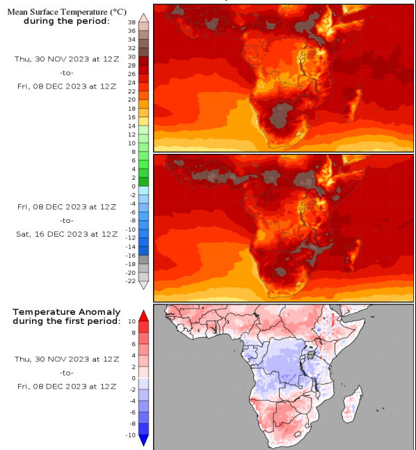
Temperature forecasts from the National Centers for Environmental Prediction. Normal Temperature derived from CRU monthly climatology for 1901-2000 Forecast Initialization Time: 12Z30NOV2023
