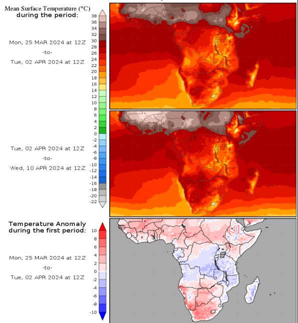
Temperature forecasts from the National Centers for Environmental Prediction. Normal Temperature derived from CRU monthly climatology for 1901-2000 Forecast Initialization Time: 12Z25MAR2024
