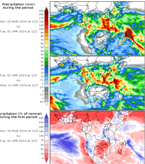
Precipitation forecasts from the National Centers for Environmental Prediction. Normal rainfall derived from Xie-Arkin (CMAP) Monthly Climatology for 1979-2003. Forecast Initialization Time: 12Z25MAR2024
