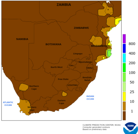
SOUTH AFRICA Total Precipitation(mm) June 9 - 15, 2024
