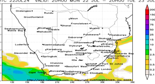
GFS 50KM POSSIBLE 24-HOUR RAINFALL (mm) INIT: 18UTC 22JUL24 VALID: 20H00 MON 22 JUL - 20H00 TUE 23 JUL
