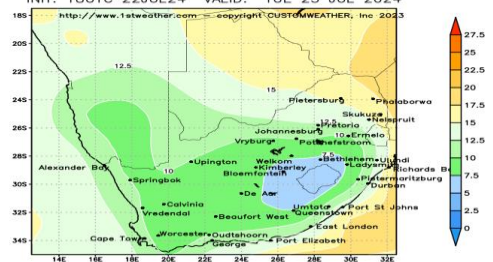
GFS 50KM MAXIMUM TEMPERATURE (C) INIT: 18UTC 22JUL24 VALID: TUE 23 JUL 2024
