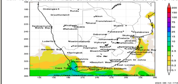
GFS 50KM POSSIBLE 24-HOUR RAINFALL (mm) INIT: 18UTC 12AUG24 VALID: 20H00 MON 12 AUG - 20H00 TUE 13 AUG
