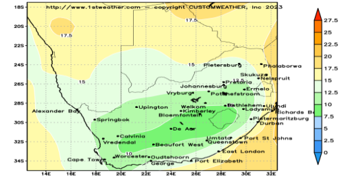
GFS 50KM MAXIMUM TEMPERATURE (C) INIT: 18UTC 12AUG24 VALID: TUE 13 AUG 2024
