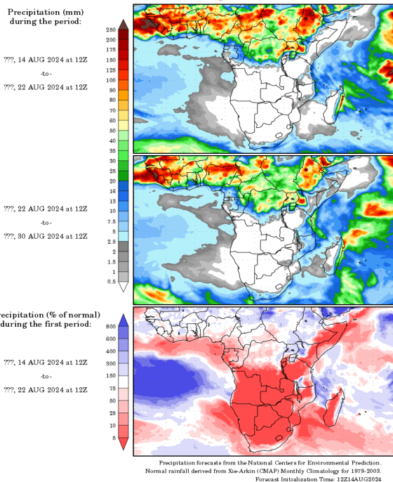
Precipitation Forecasts
