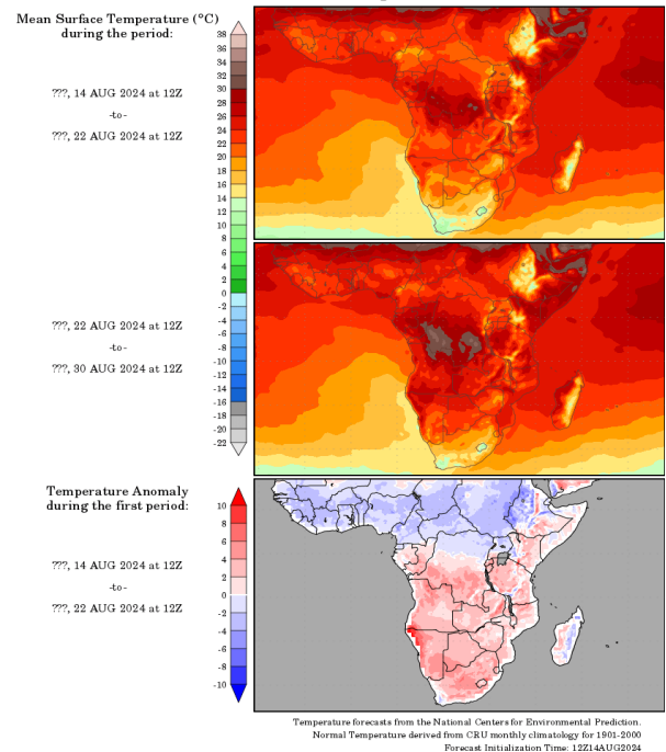
Temperature Forecasts
