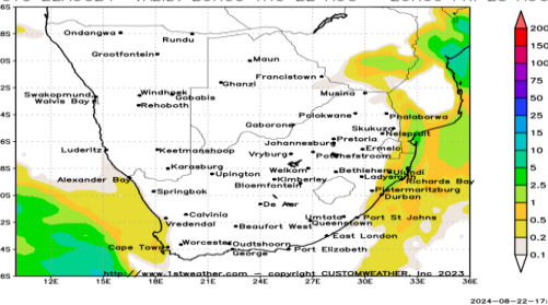
GFS 50KM POSSIBLE 24-HOUR RAINFALL (mm) INIT: 18UTC 22AUG24 VALID: 20H00 THU 22 AUG - 20H00 FRI 23 AUG
