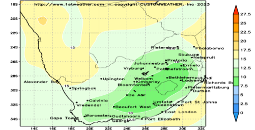
GFS 50KM MAXIMUM TEMPERATURE (C) INIT: 18UTC 22AUG24 VALID: FRI 23 AUG 2024
